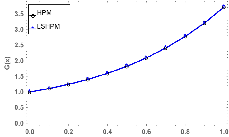
Figure 3: Comparison of solutions in Problem 2.
