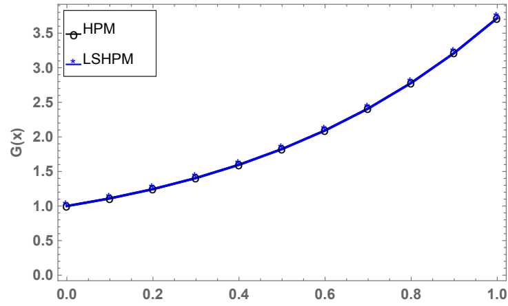
Figure 7: Comparison of solutions in Problem 4.
