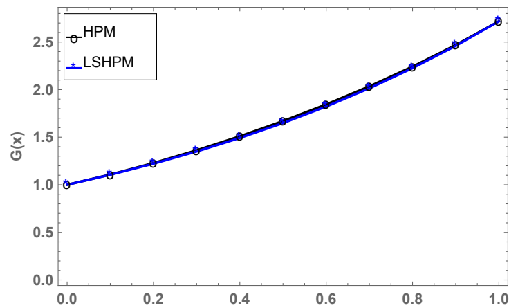
Figure 9: Comparison of solutions in Problem 5.
