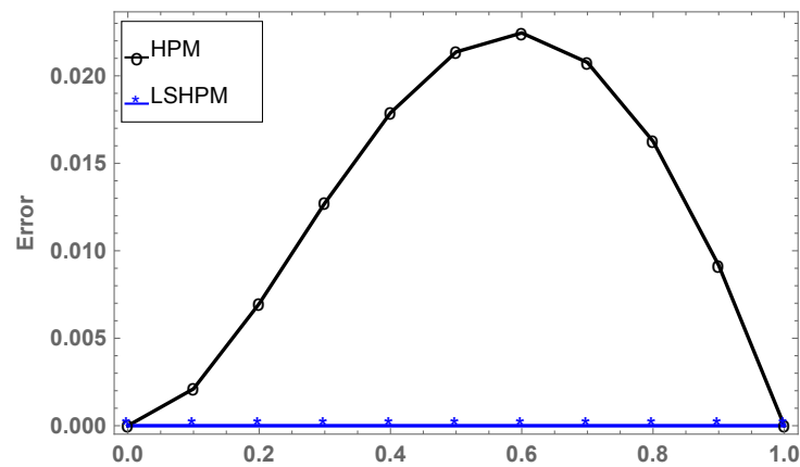
Figure 10: Comparison of errors in Problem 5.
