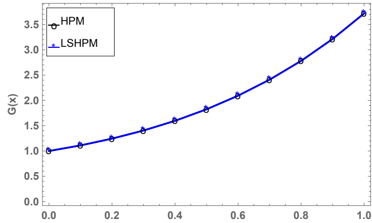
Figure 1: Comparison of solutions in Problem 1.
