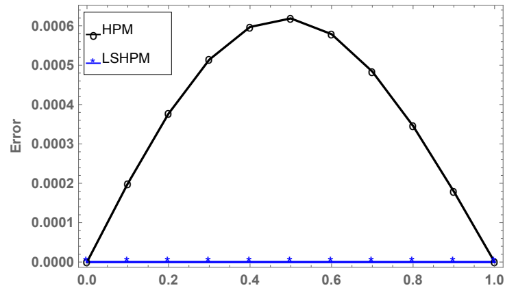
Figure 2: Comparison of errors in Problem 1.
